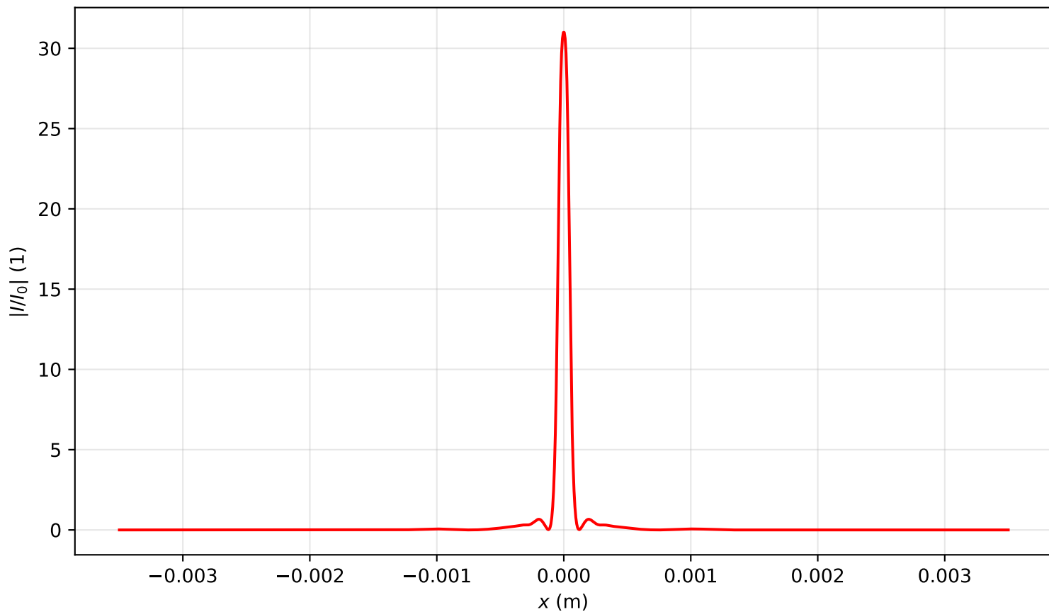
Intensity profile I(x, y = 0, z = 1.433)/I_0 , P_{in}=3.5P_{cr} , artificial time
